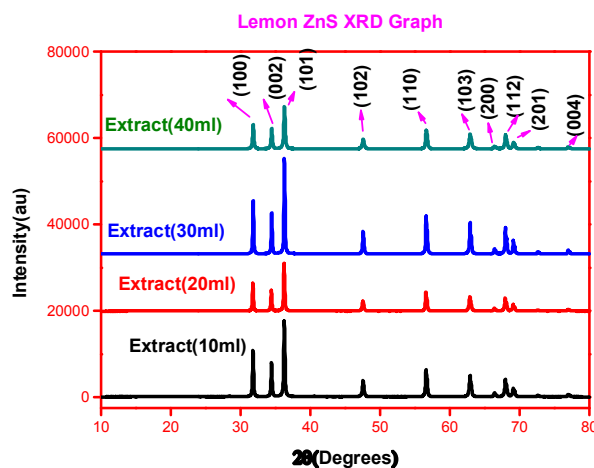
Fig. 1. XRD of Lemon ZnO nanoparticles
