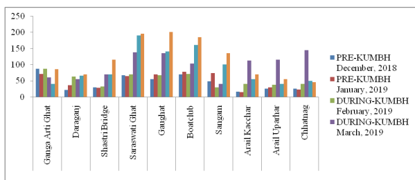
Fig. 8. Effect of Kumbh Mela on chloride (mg/l) of water quality of river Ganga and Yamuna at Prayagraj 2019
