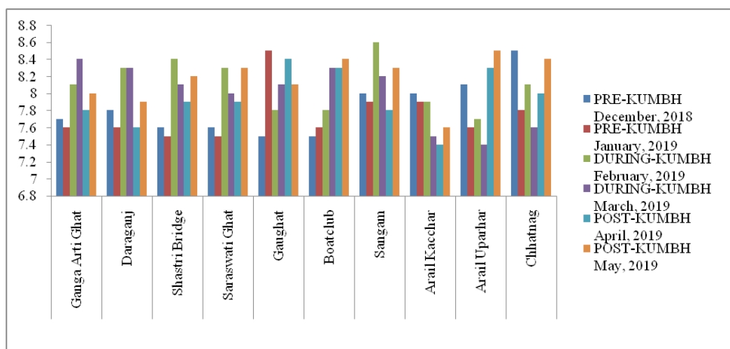
Fig. 1. Effect of Kumbh Mela on the pH of water quality of river Ganga and Yamuna at Prayagraj 2019
