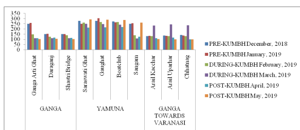
Fig. 3. Effect of Kumbh Mela on TDS ( \text{mg/l} ) of water quality of river Ganga and Yamuna at Prayagraj 2019
