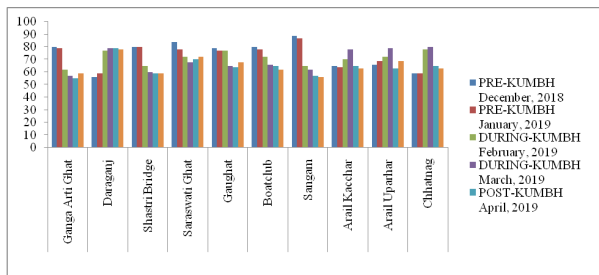
Fig. 7. Effect of Kumbh Mela on alkalinity (mg/l) of water quality of river Ganga and Yamuna at Prayagraj 2019
