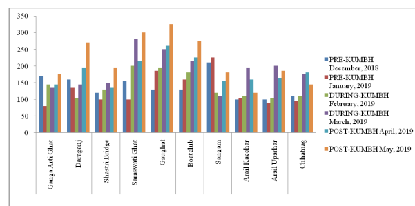
Fig. 5. Effect of Kumbh Mela on calcium hardness ( \text{mg/l} ) of water quality of river Ganga and Yamuna at Prayagraj 2019
