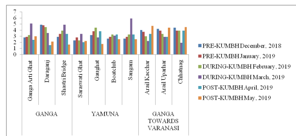
Fig. 10. Effect of Kumbh Mela on BOD (mg/l) of water samples of river Ganga and Yamuna at Prayagraj 2019
