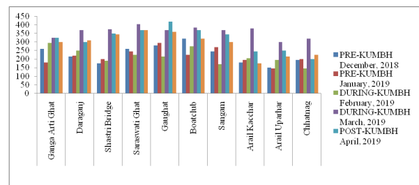
Fig. 4. Effect of Kumbh Mela on total hardness ( \text{mg/l}^{-1} ) of water quality of river Ganga and Yamuna at Prayagraj 2019
