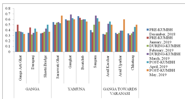
Fig. 2. Effect of Kumbh Mela on EC ( \text{dSm}^{-1} ) of water quality of river Ganga and Yamuna at Prayagraj 2019
