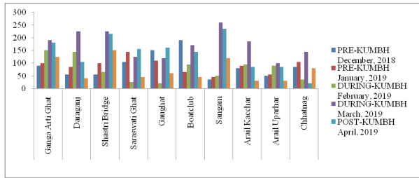
Fig. 6. Effect of Kumbh Mela on Mg hardness (mg/l) of water quality of river Ganga and Yamuna at Prayagraj 2019
