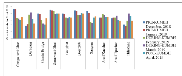
Fig. 9. Effect of Kumbh Mela on DO (mg/l) of water quality of river Ganga and Yamuna at Prayagraj 2019
