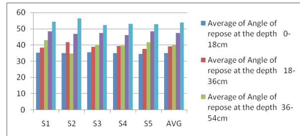
Fig. 3. Angle of repose of FYM at different depth of manure pit
