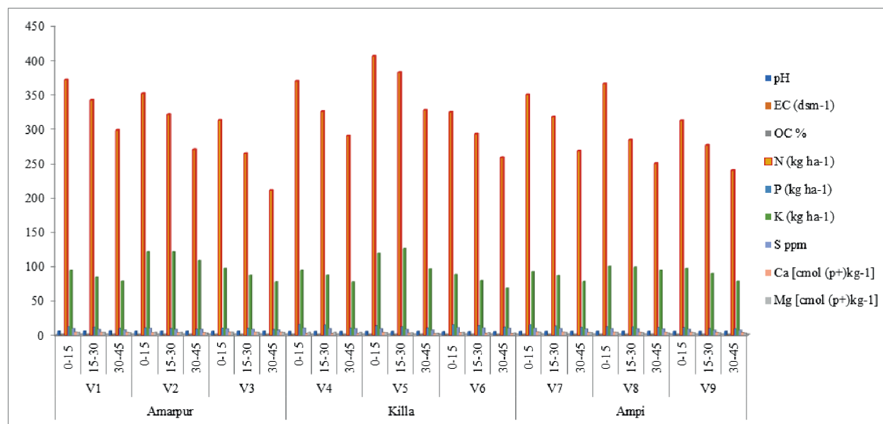
Fig. 1. Showing Variation in Chemical Parameters of soil samples of Gomati district, Tripura.
